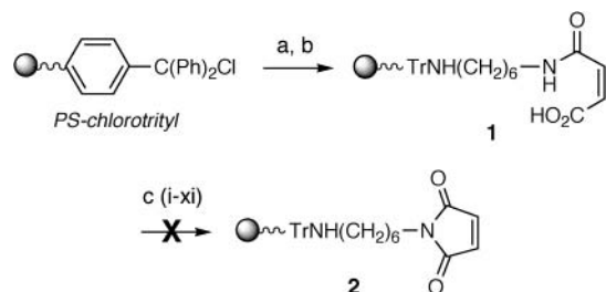
Scheme 1. Attempted Cyclative Dehydration Routes to Cleavable Resin-Supported N -Alkylmaleimides a
