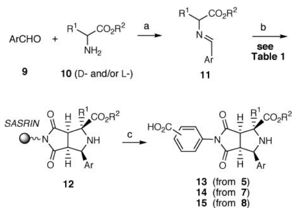
Scheme 3. 1,3-Dipolar Cycloaddition between Azomethine Ylids of \alpha -Iminoesters 11 and SASRIN MBA Resins 5 , 7 , and 8 a
