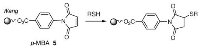
Scheme 4. Scavenging of Sulfhydryl Compounds with Wang p -MBA Resin 5 a
