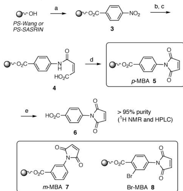
Scheme 2. General Route for the Preparation of N -Arylmaleimidobenzoic Acid (MBA) Resins a
